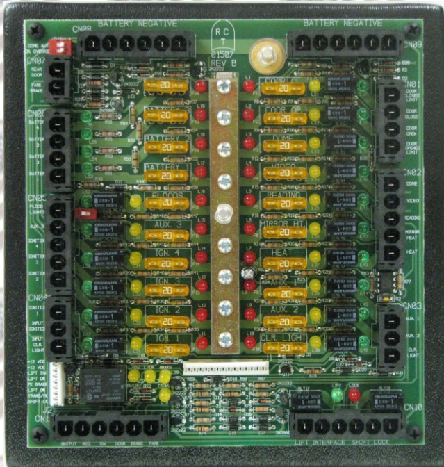
RCT-015070-00000, Bus Power Center Control Size: Top to Bottom 7.50" Left to Right 8"
